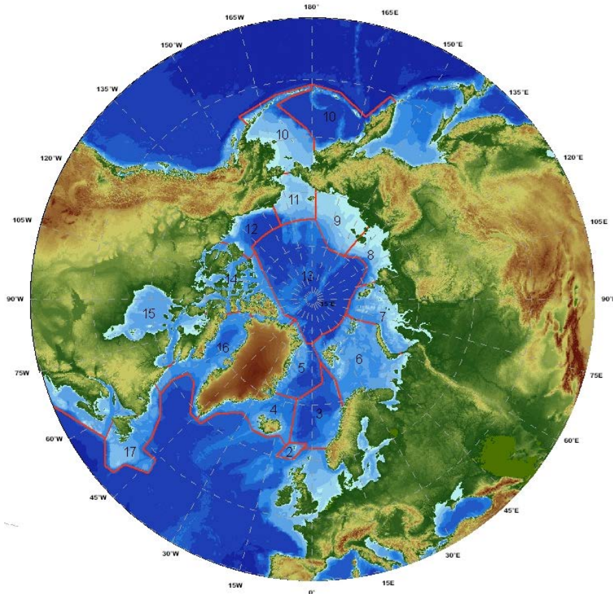
Figure 2. Adjusted 2006 LME working map used in the 2007 Assessment of Arctic oil and gas activities.
