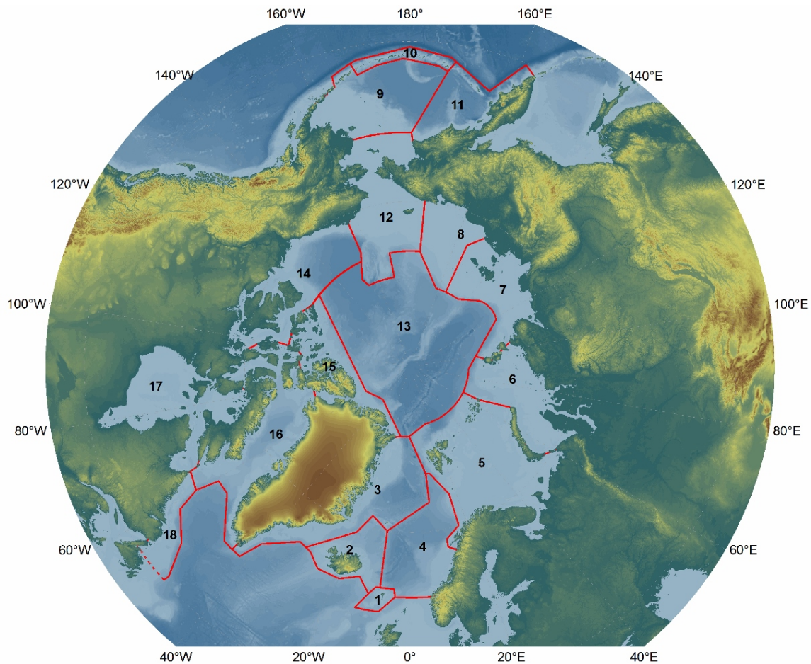
Figure 3. Revised Map of 18 Arctic LMEs (version 17 April 2013).
