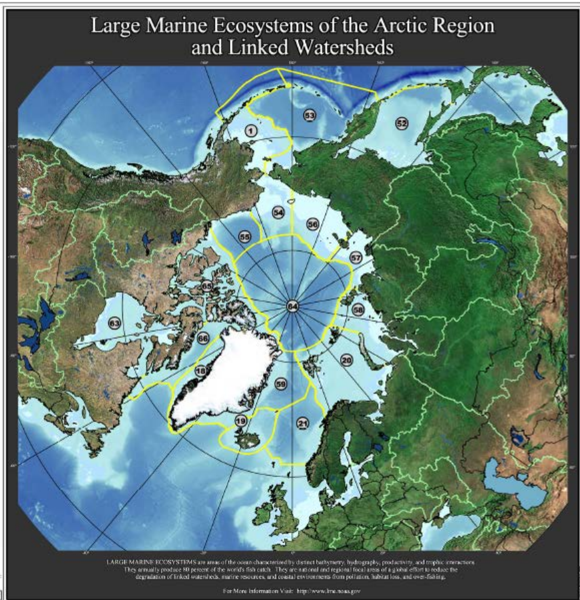
Figure 1. Working map of Arctic Large Marine Ecosystems (LMEs) from 2006.
